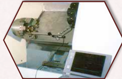
Ball Bar Test for Checking Dynamic Performance of M/c
