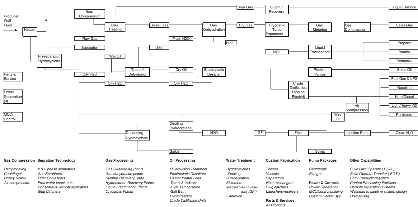
Process Diagram
